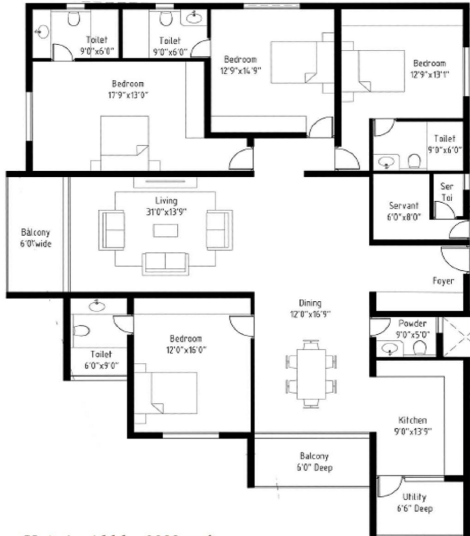
Unit A - 4 bhk - 3000 sq.ft
