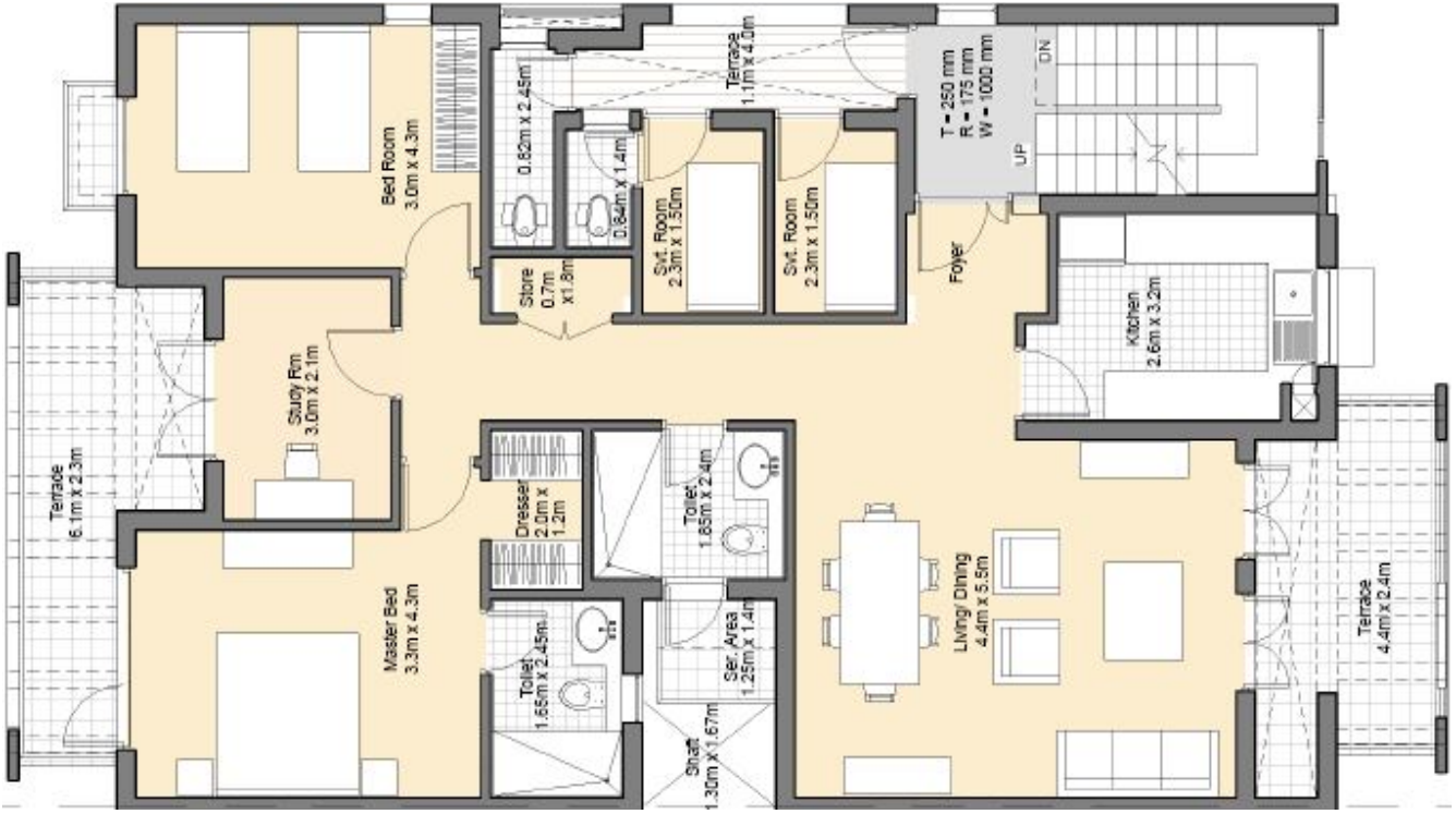
Second Floor Unit Area:1755.72 Sq.Ft
