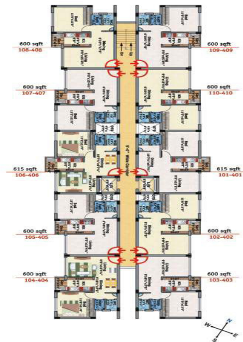
Typical Floor Plan Towers - A5 (4 Floors)
