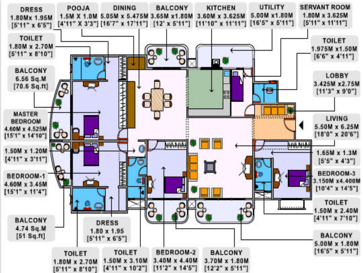
A1 Block Typical Floor Plan
