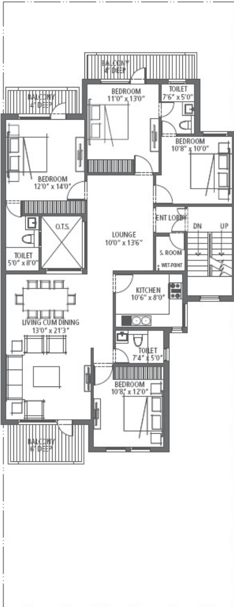
First & Second Floor Plan
