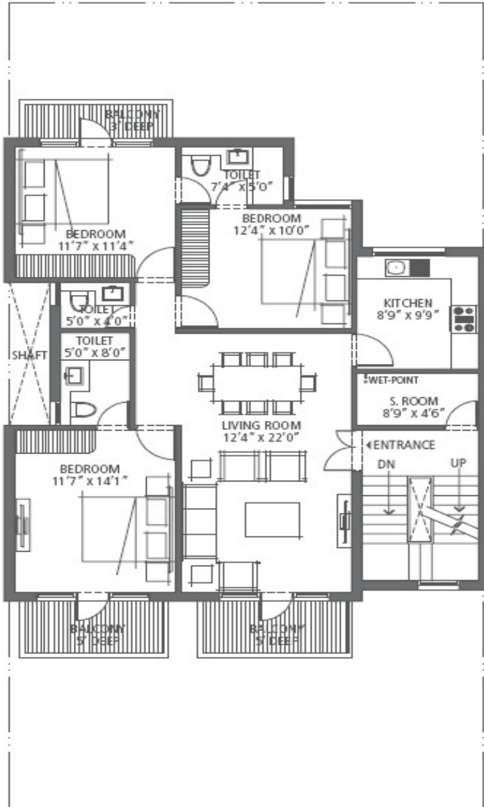
First & Second Floor
