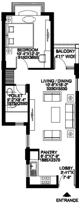
TENTATIVE PLAN OF APARTMENT NO. 1,4,5 & 8 (NOT TO SCALE)
