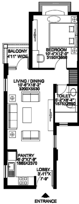
TENTATIVE PLAN OF APARTMENT NO. 2 & 3
