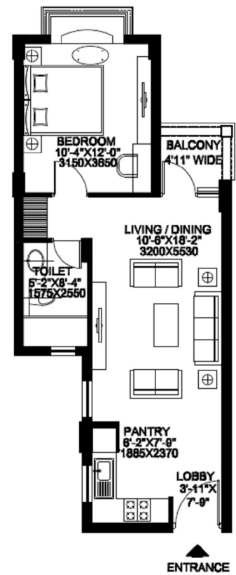
TENTATIVE PLAN OF APARTMENT NO. 6 & 7
