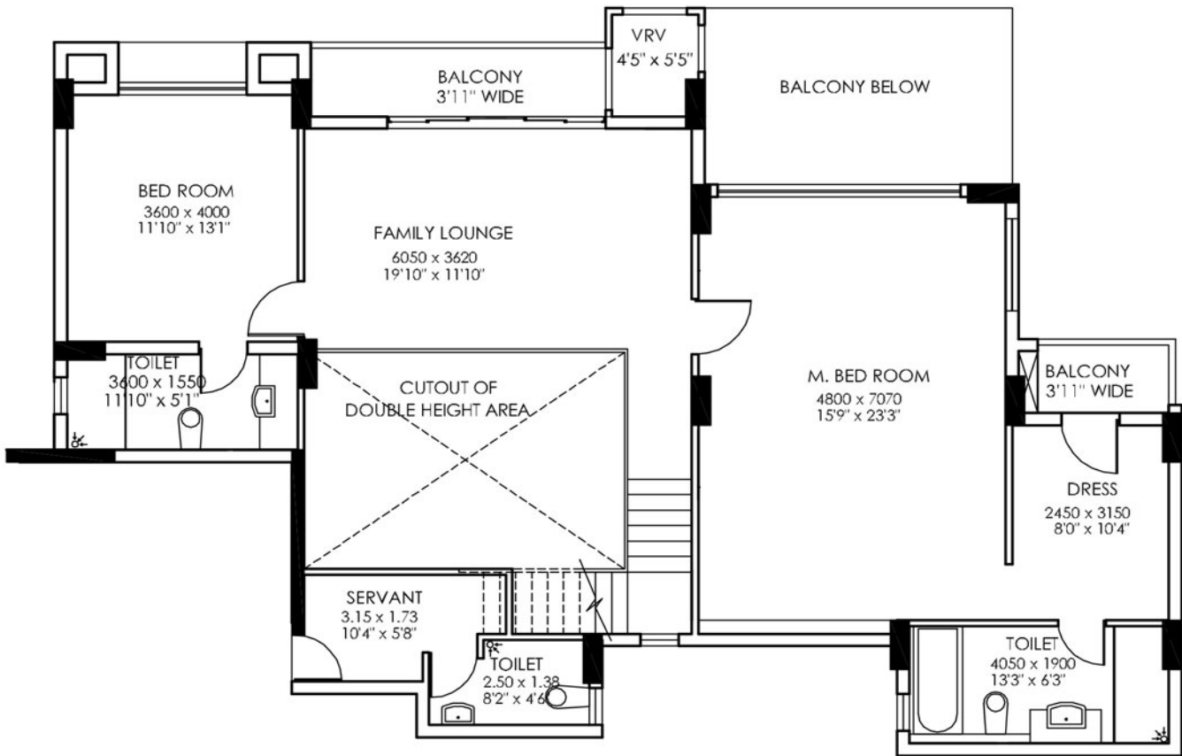
TENTATIVE UPPER LEVEL PLAN OF DUPLEX - 1 & 4
