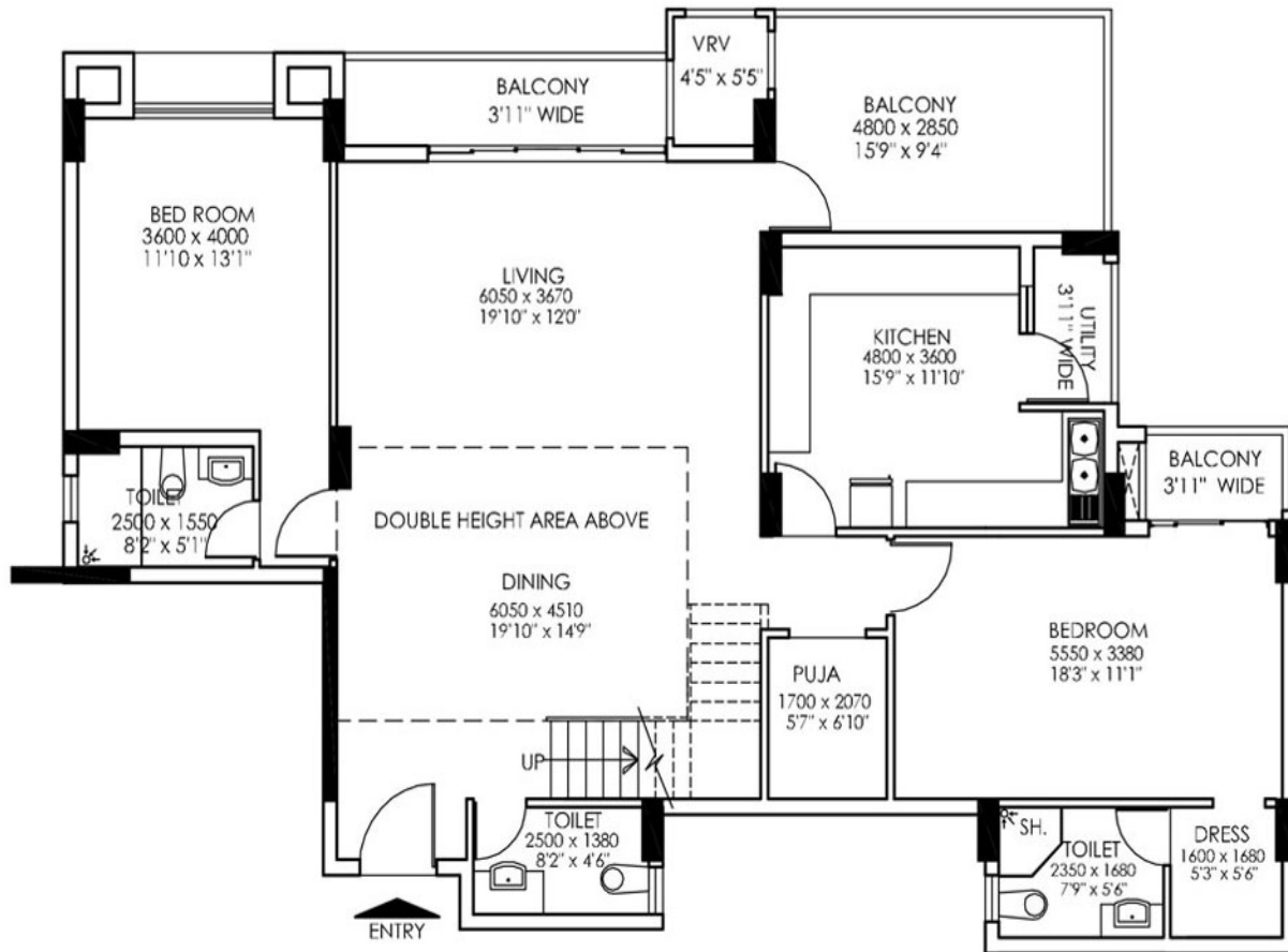
TENTATIVE LOWER LEVEL PLAN OF DUPLEX - 1 & 4 TENTATIVE SALEABLE AREA = 3957 SQFT
