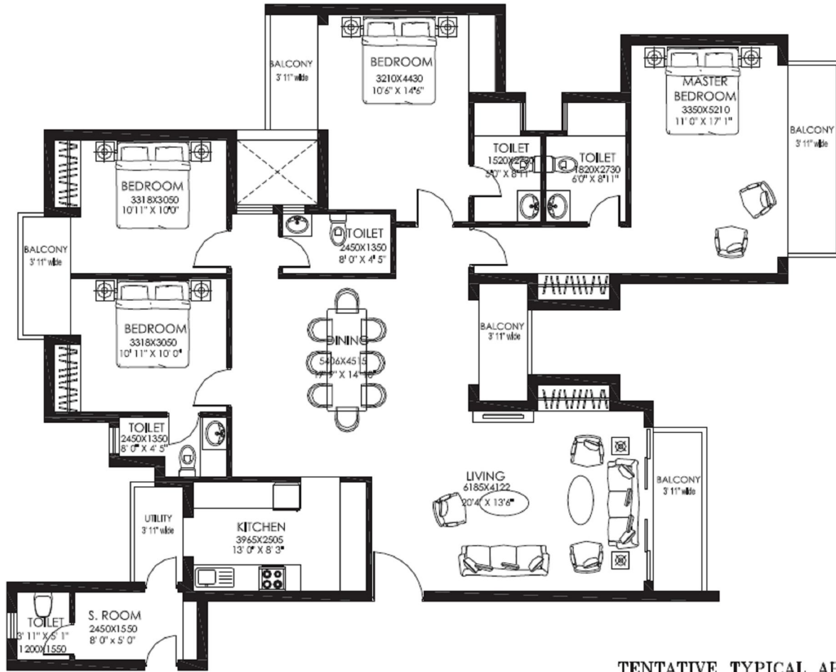
TENTATIVE TYPICAL APARTMENT PLAN
